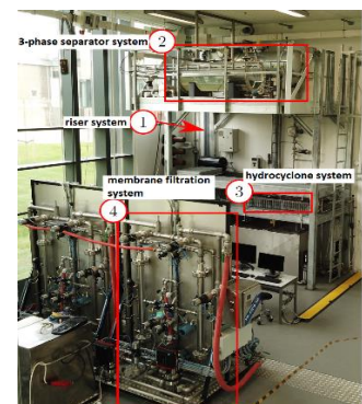
AAU water treatment pilot-plant
