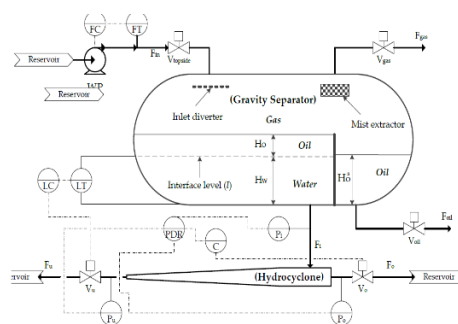
Hydrocyclone coupled with separator and controls
