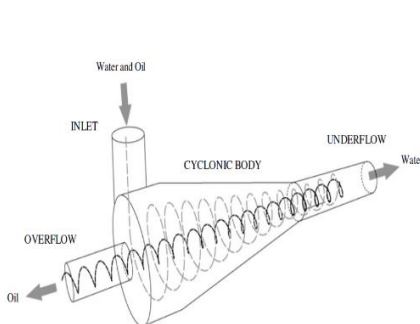
Single hydrocyclone configuration
